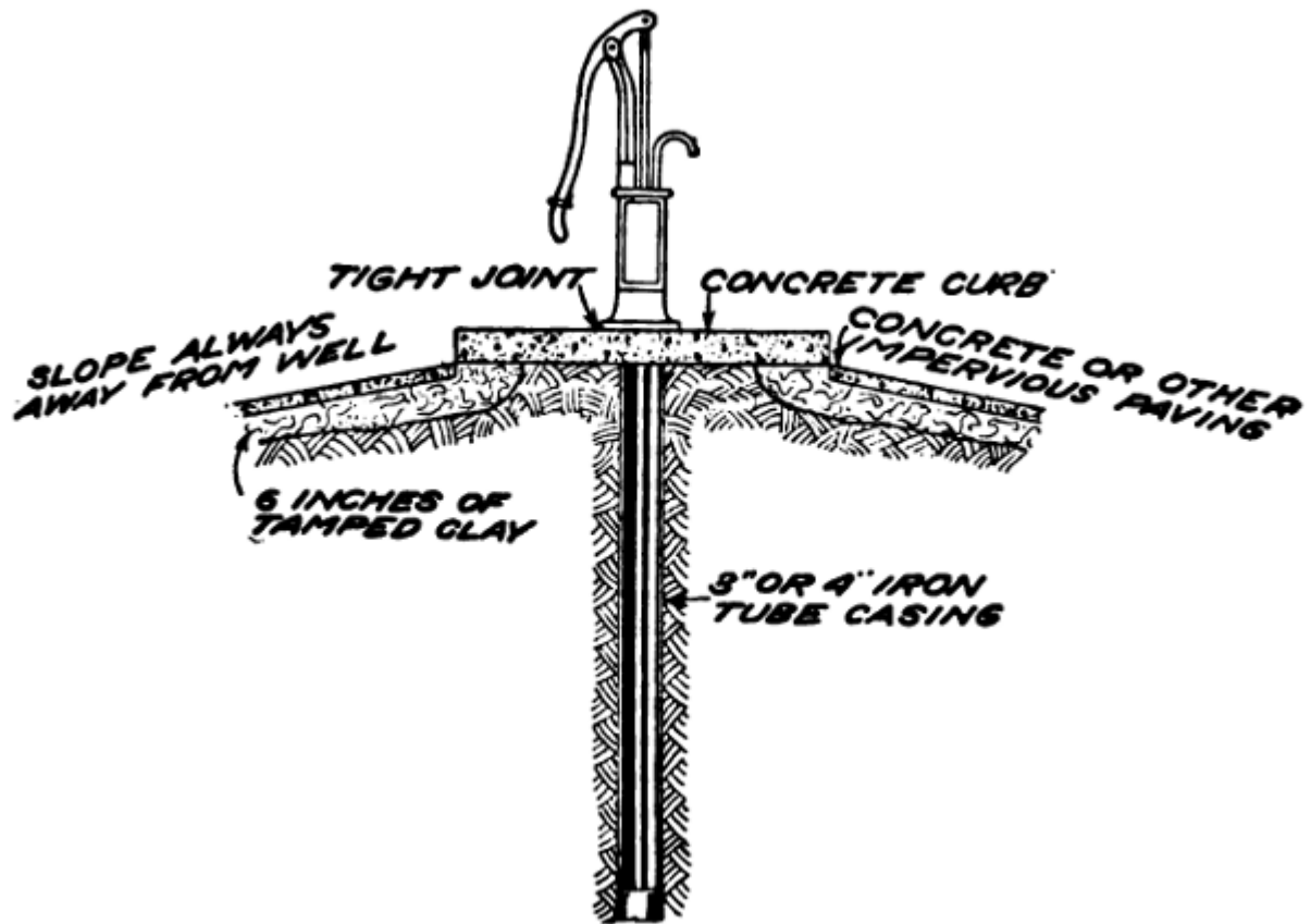
Fig. 19.—Bored well.
