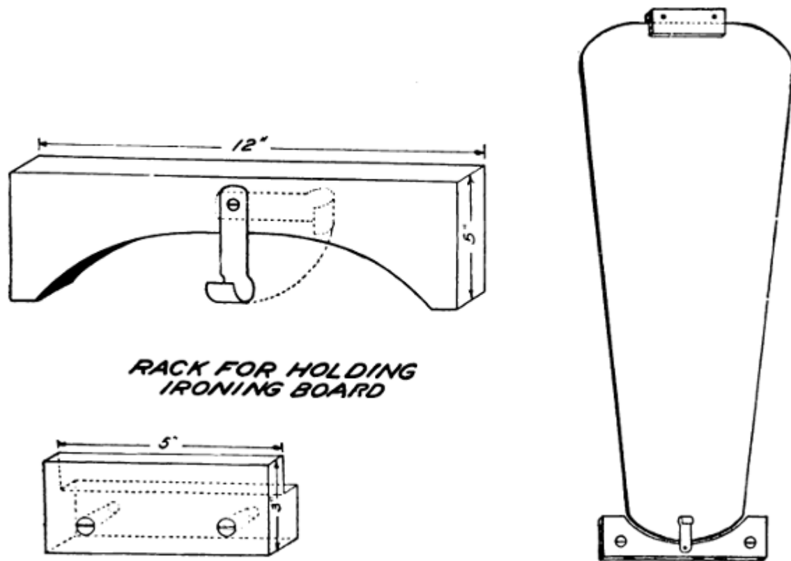
Fig. 10.—Rack for holding ironing board.
