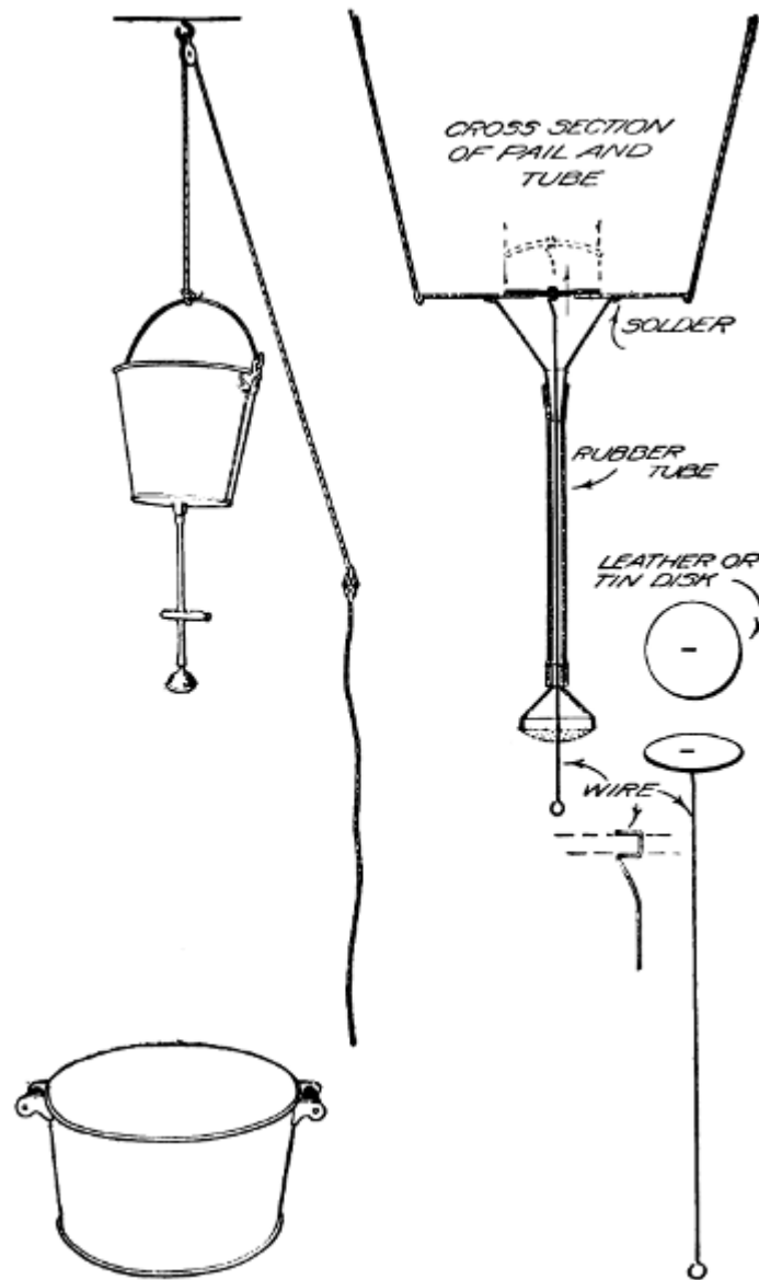
Fig. 16.—The shower bath.
