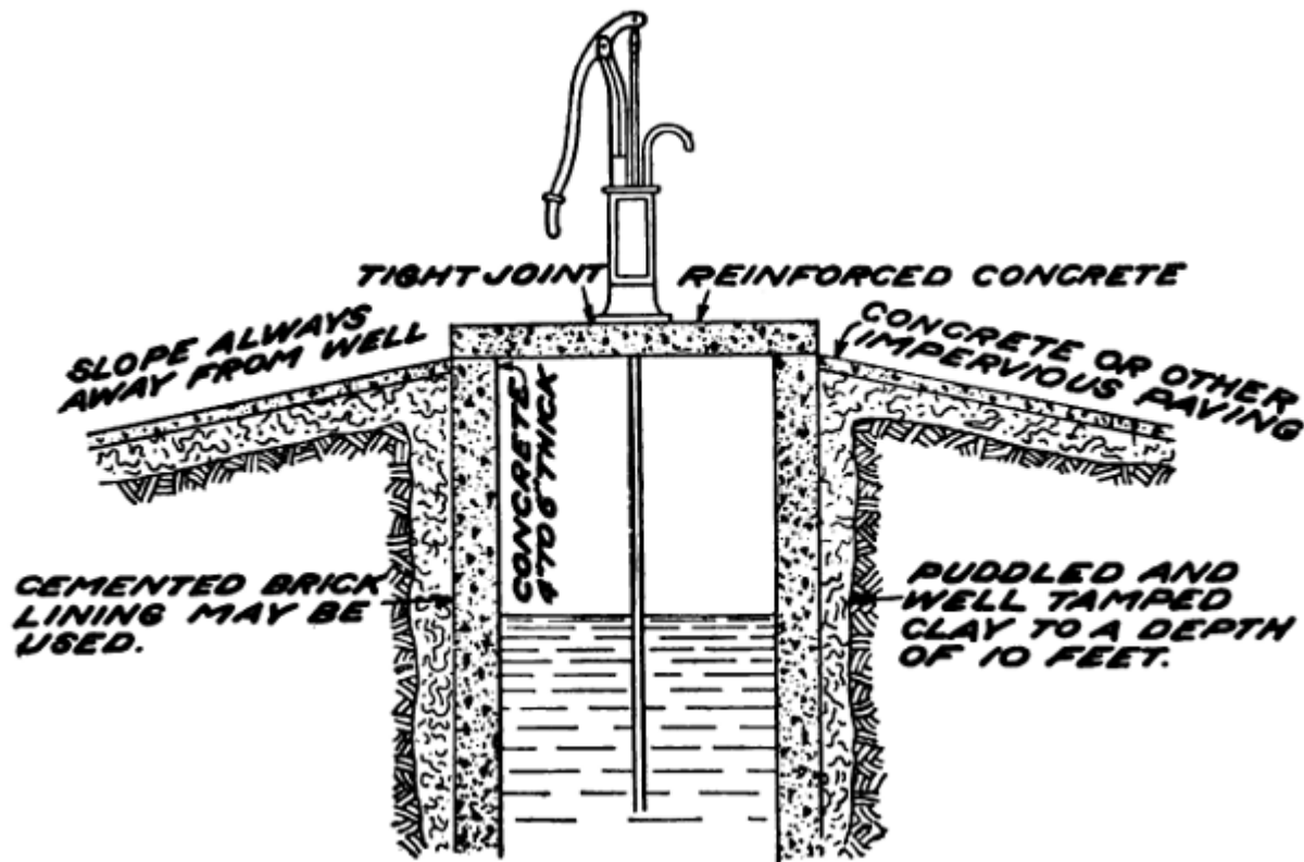
Fig. 17.—Dug well, concrete or cemented-brick lining.
