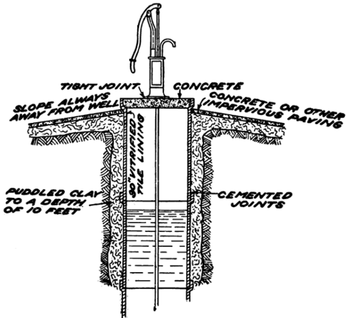
Fig. 18.—Dug well, vitrified tile lining.
