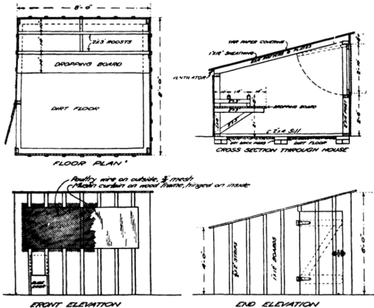
Fig. 6.—Plan of a simple back-yard poultry house.
