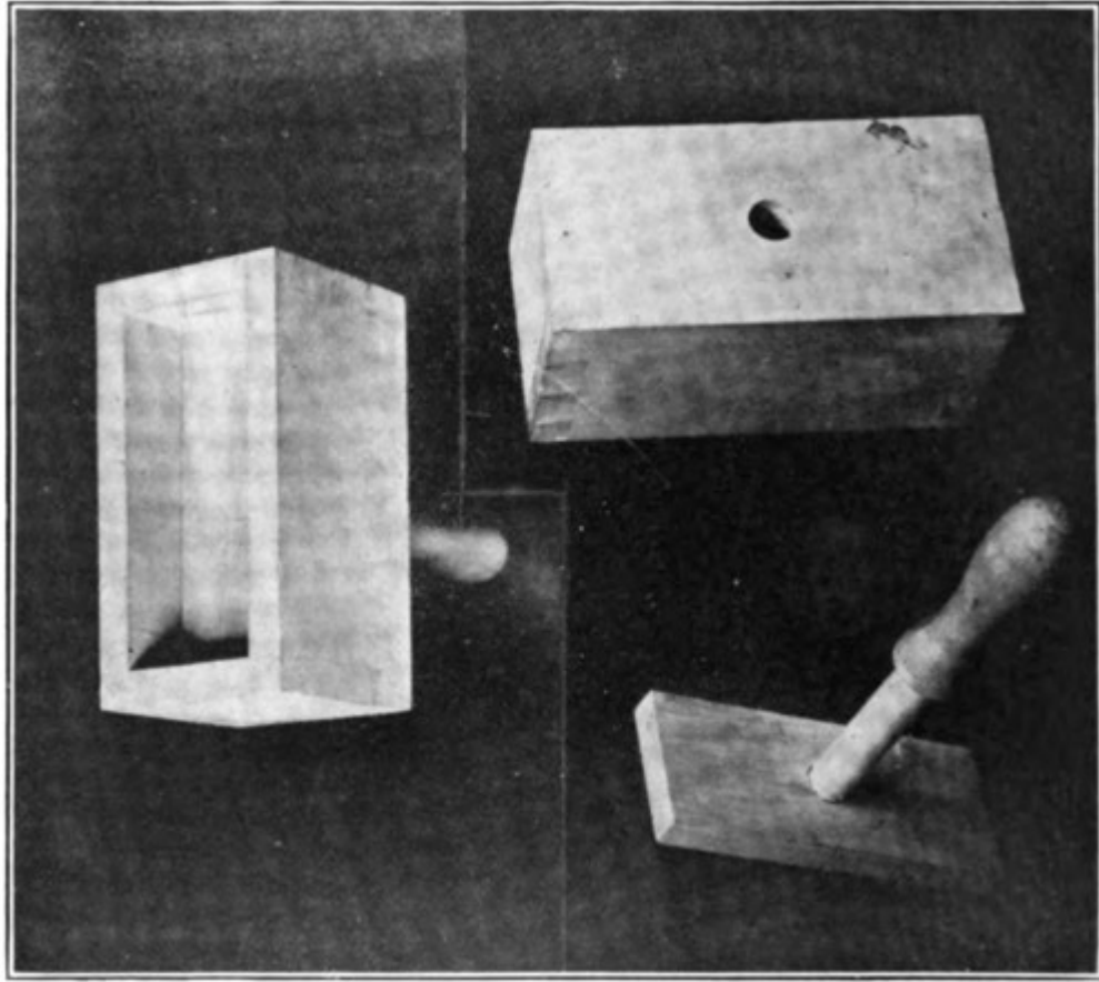
Fig. 1.—Two views of hand printer for 1-pound prints.
