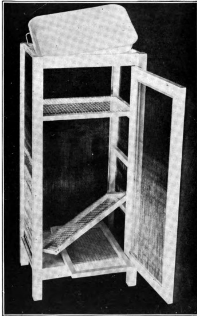
Fig. 11.—Framework of the iceless refrigerator.
