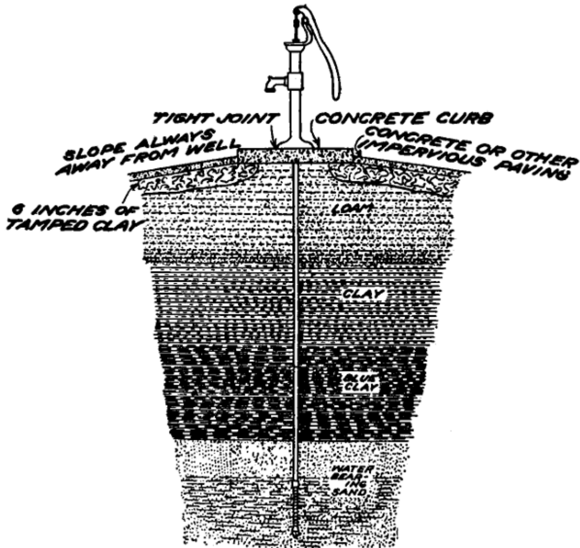
Fig. 20.—Driven well.
