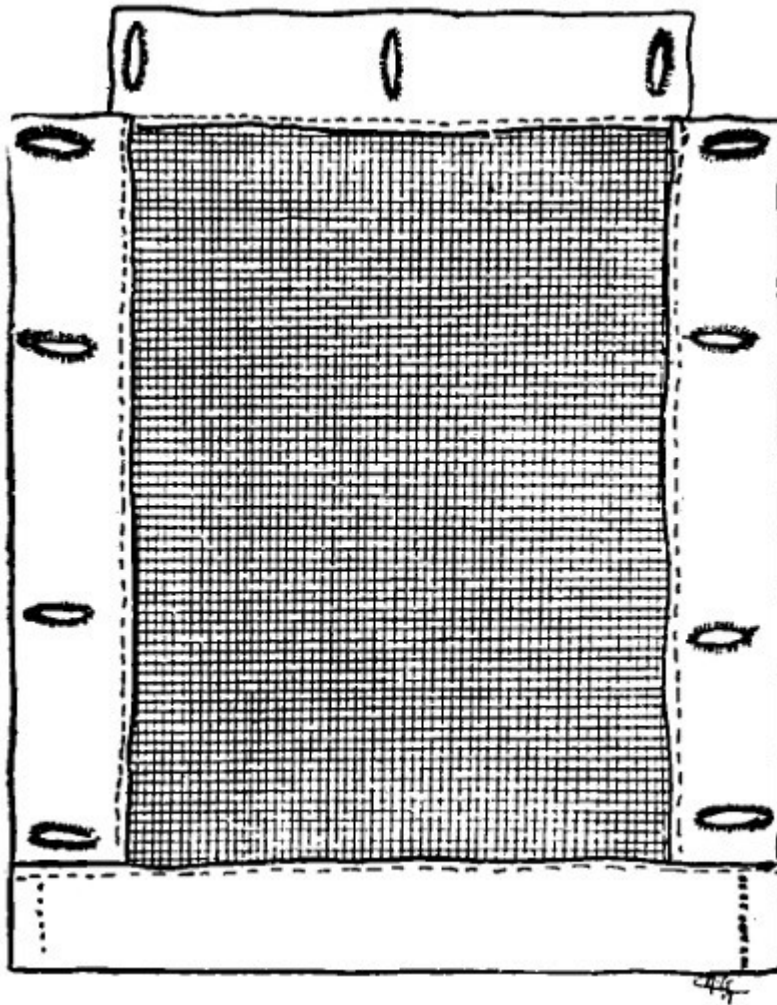
Fig. 23.—Window screen.
